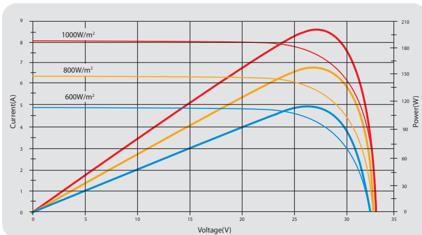
Current-Voltage & Power-Voltage Curve (200W)
